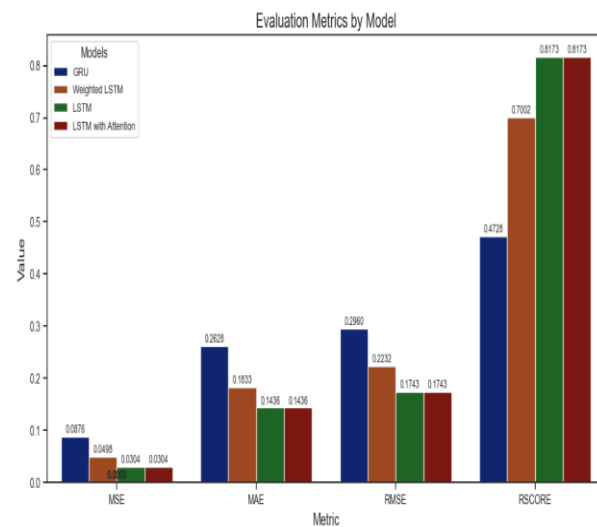
Figure 6: Plot of evaluation
