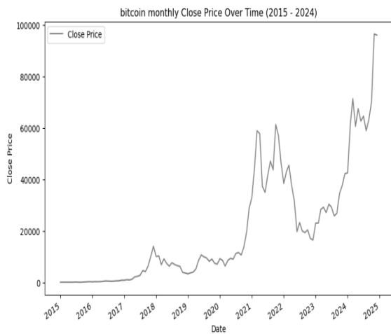
Figure 2: BTC monthly close price (2015-2024)
