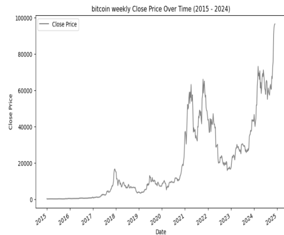
Figure 3: BTC weekly close price (2015-2024).
