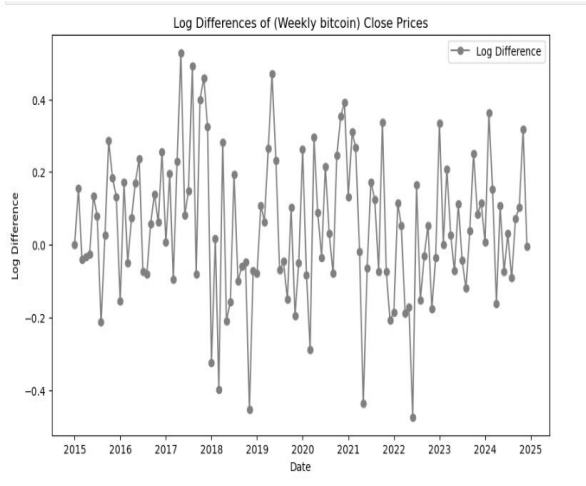
Figure 4: Log difference of BTC monthly close price.
