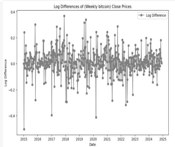
Figure 5: Log difference of BTC weekly close price.
